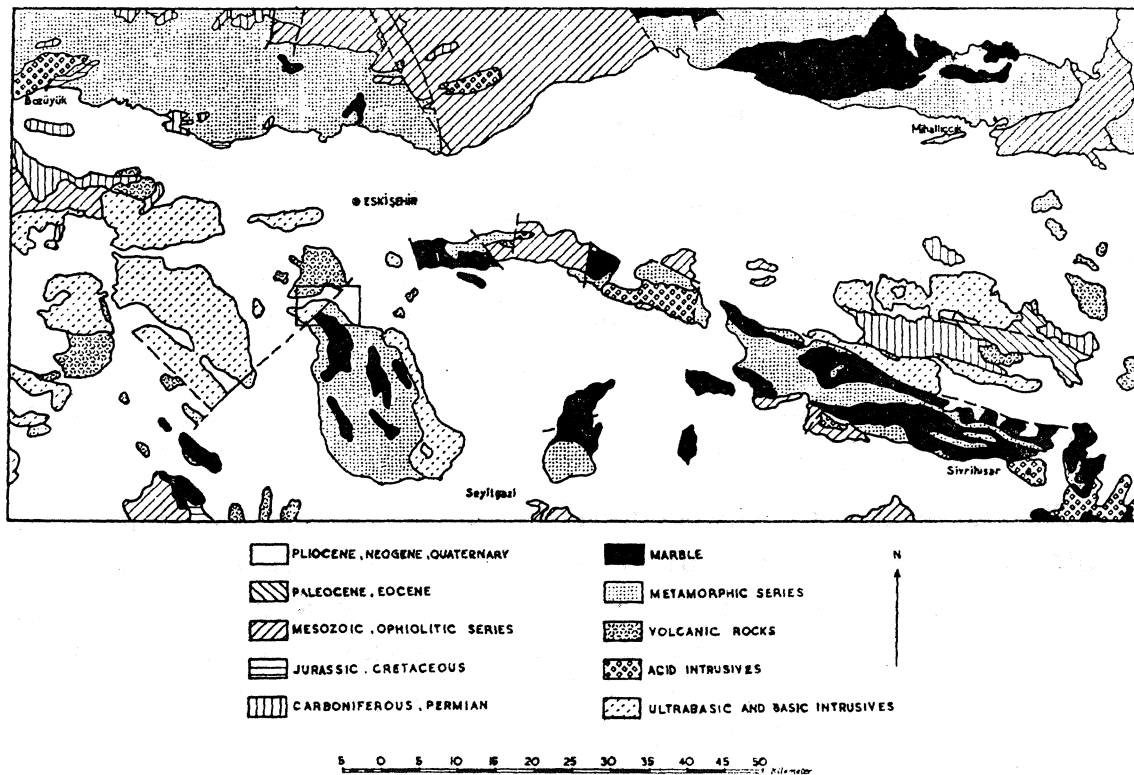
Fig. 2. GEOLOGICAL MAP OF ESKİŞEHİR AREA (Northwest of ANKARA Sheet).
