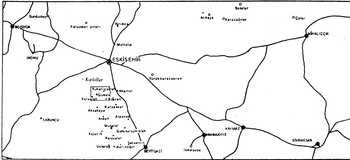
Fig. 1. LOCALITY MAP OF ESKİŞEHİR AREA
